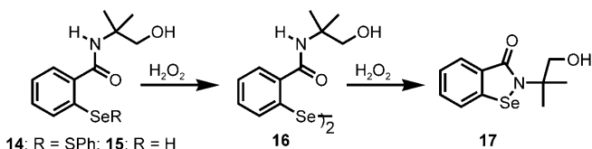
Scheme 7. The formation of diselenide 16 and the cyclic selenenyl amide 17 from compounds 14 and 15 .
